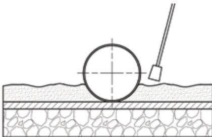
Fig. 17: Proper backfilling at the haunches
