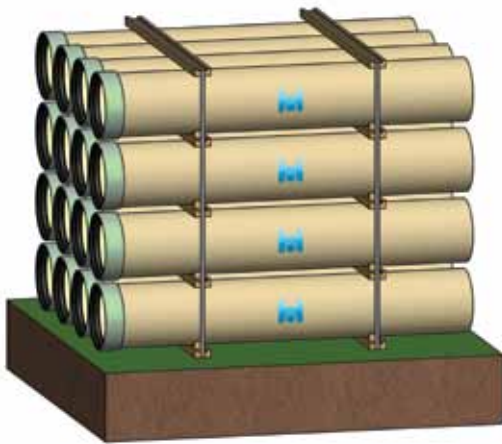
Fig. 7: Packaging unit
