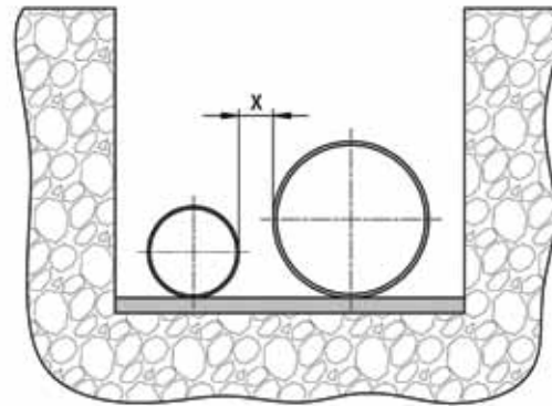
Fig. 10: Minimum spacing (x) between pipelines
