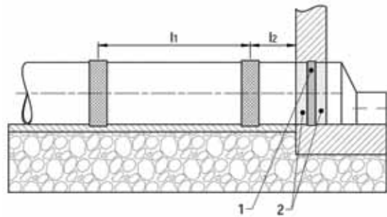
Fig. 37: Connection to buildings with structural adapters
