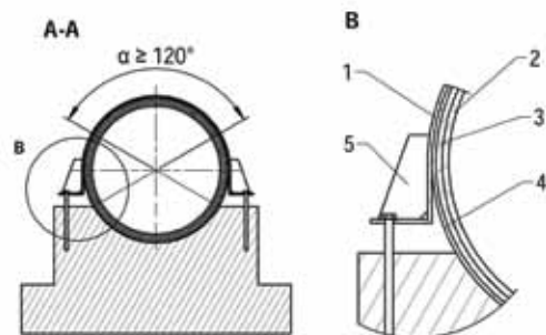
Fig. 27: Above-ground support at the coupling, cross-section
