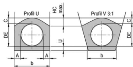
Fig. 59: Trench shapes acc. to SIA V190
