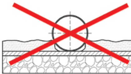
Fig. 16: Inadequate backfilling at the haunches
