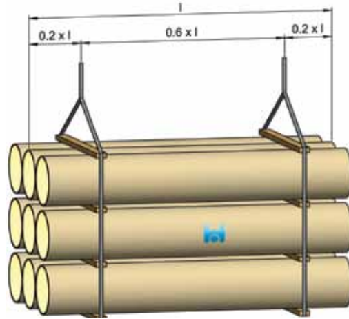
Fig. 1: Packaging units
